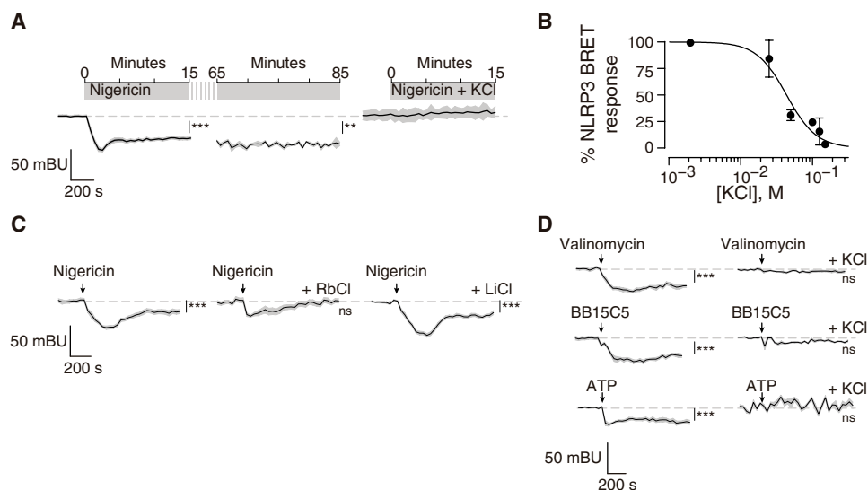
Fig. 2. K^+ efflux modifies the NLRP3 structure. (A) Average BRET signal for YFP-NLRP3-Luc expressed in HEK293T cells before and after stimulation with nigericin (10 \mu M, denoted by a gray box) in the absence (left, middle) or presence (right) of 140 mM KCl; note that kinetics of BRET have been plotted with the same scale, but relatively at the same level to ease comparison. n = 51, 4, and 6 for nigericin 15 min, nigericin 85 min, and nigericin + KCl, respectively; Mann-Whitney test. (B) NLRP3 BRET signal variation after treatment for 15 min with nigericin (10 \mu M) versus basal conditions without nigericin in the presence of increasing concentrations of KCl. n = 3 to 5 independent cell culture wells for each KCl concentration. (C) Average BRET signal for YFP-NLRP3-Luc expressed in HEK293T cells before and after stimulation with nigericin (10 \mu M) in the absence/presence of 40 mM RbCl or 40 mM LiCl; note that kinetics of BRET have been plotted with the same scale, but relatively at the same initial level to ease comparison. n = 12 independent cultures from four independent experiments; Mann-Whitney test. (D) Average BRET signal for YFP-NLRP3-Luc expressed in HEK293T cells (top and middle) or HEK293T-P2X7 receptor (bottom), before and after stimulation with valinomycin (50 \mu M), BB15C5 (50 \mu M), or ATP (3 mM), in the absence/presence of 140 mM KCl; note that kinetics of BRET have been plotted with the same scale, but relatively at the same initial level to ease comparison. n = 6 to 18 independent cell cultures; Mann-Whitney test.
